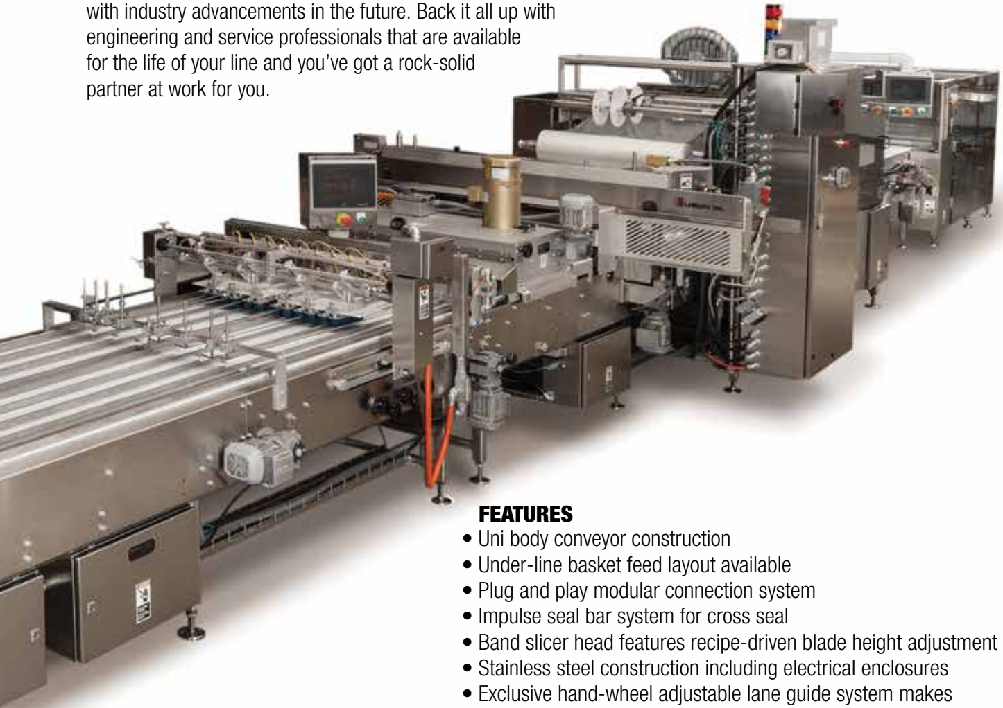
LS133 shown with optional Hinge Slicer and Band Slicer and Tray Loader
